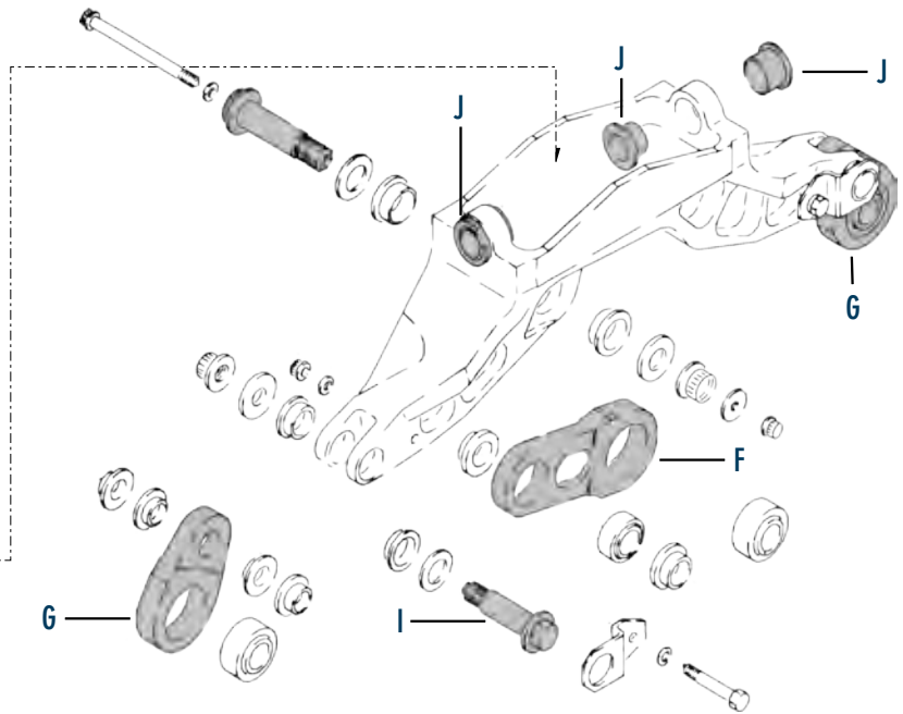
Aft Engine Mount Assembly 310N3020 - All Series
